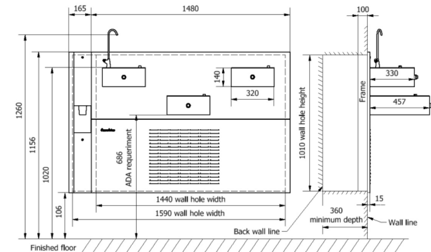
Model: EF3PVALVBA-8HET
