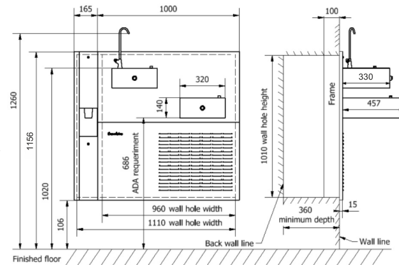
Model: EF2PVALVB-8HET
